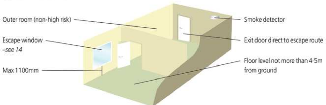
figure C3: inner rooms
